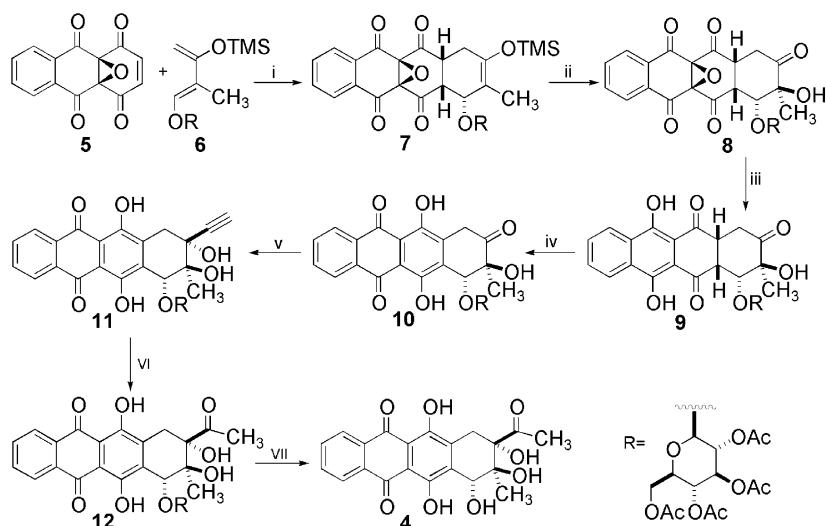
Scheme 1. (i) \text{CH}_3\text{CN} , rt, overnight; (ii) DMDO, acetone, rt, overnight; (iii) \text{Zn} , \text{AcOH} , \text{CH}_2\text{Cl}_2 , -20^\circ\text{C} , 1 h; (iv) \text{Pb}(\text{OAc})_4 , \text{AcOH} , rt, 15 h; (v) \text{HC}\equiv\text{CMgCl} , \text{THF} , 0^\circ\text{C} , 1 h; (vi) \text{HgO} , \text{H}_2\text{SO}_4 , acetone, reflux, 0.5 h; (vii) \text{HCl} , \text{C}_2\text{H}_5\text{OH} , reflux, 25 h.
